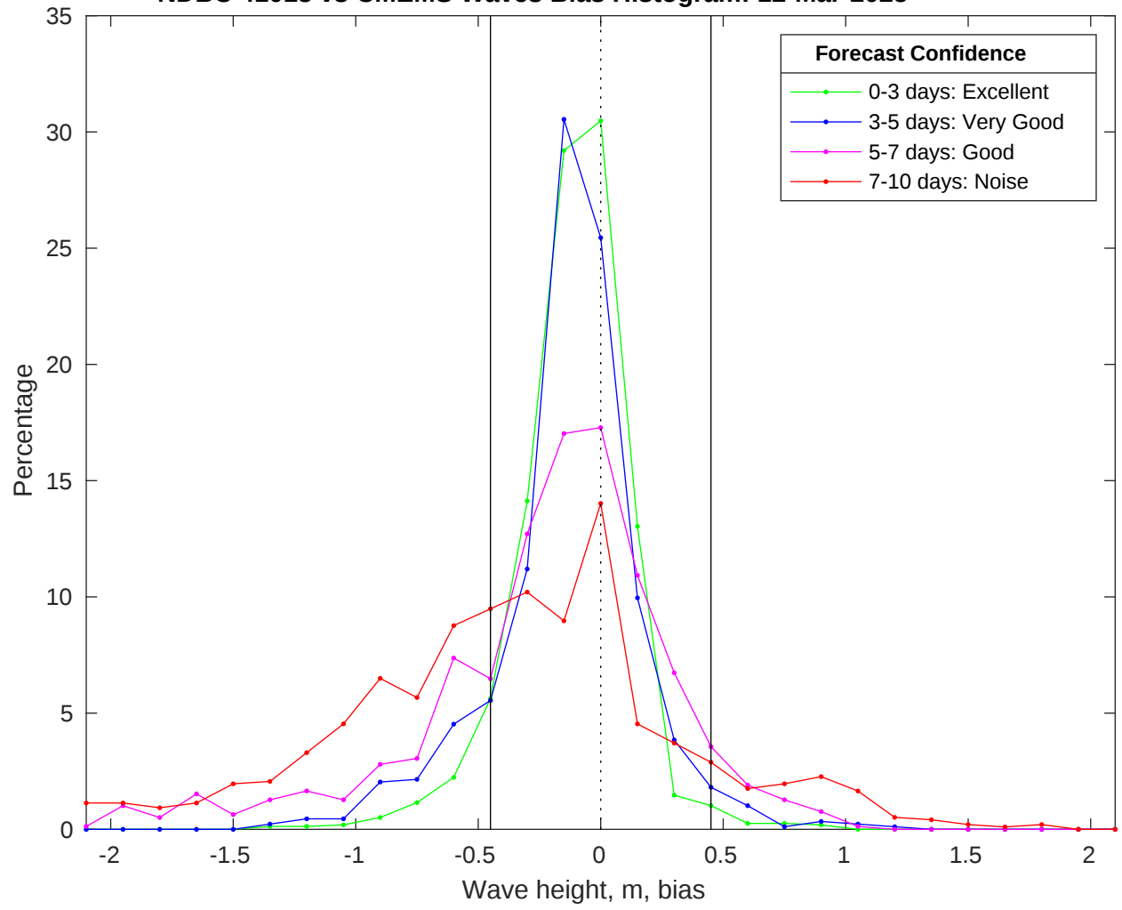
NDBC 41013 vs CMEMS Waves Bias Histogram: 12-Mar-2025
