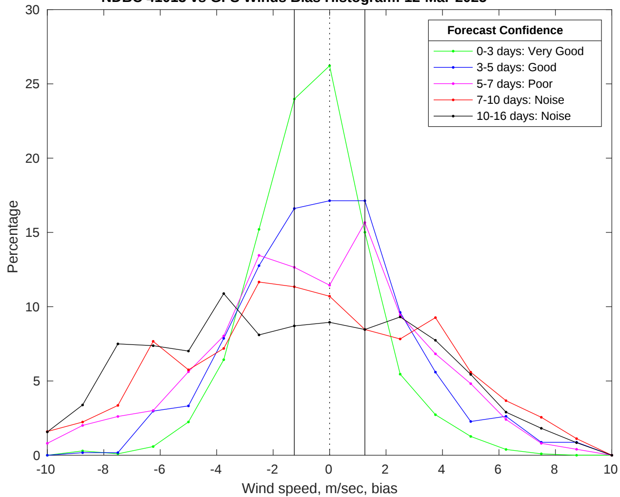
NDBC 41013 vs GFS Winds Bias Histogram: 12-Mar-2025
