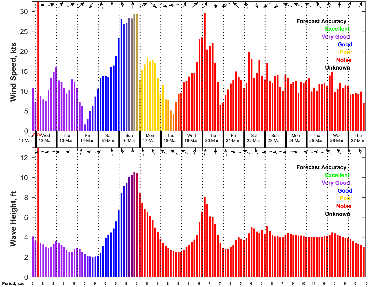
Wind & Wave Forecast for NDBC 41013 from 11-Mar-2025 19:00:00 to 27-Mar-2025 19:00:00
