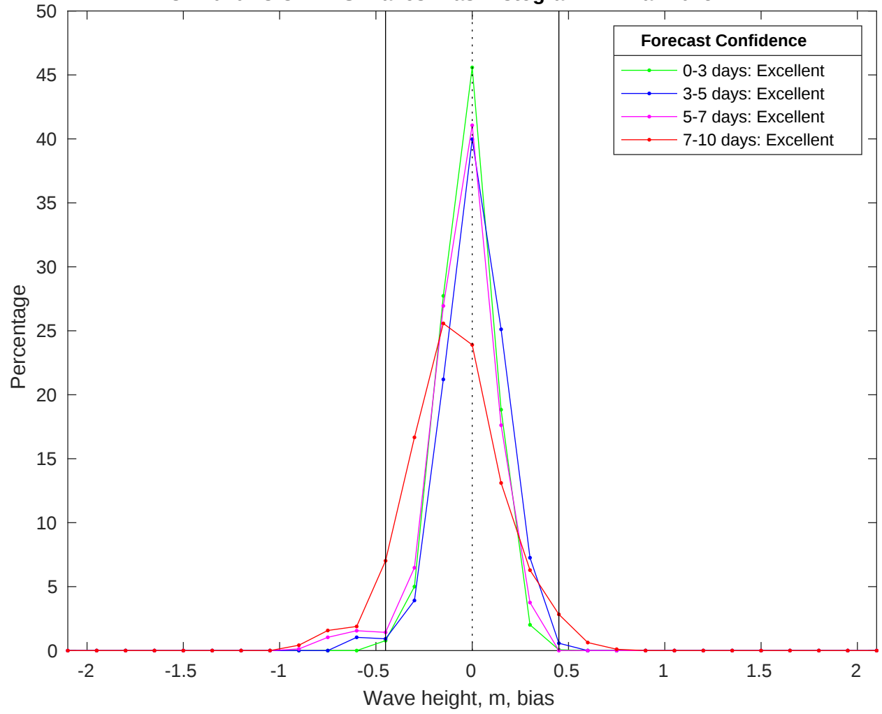
NDBC 41040 vs CMEMS Waves Bias Histogram: 12-Mar-2025
