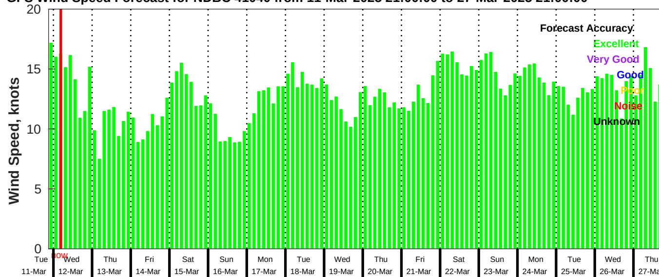
GFS Wind Speed Forecast for NDBC 41040 from 11-Mar-2025 21:00:00 to 27-Mar-2025 21:00:00
