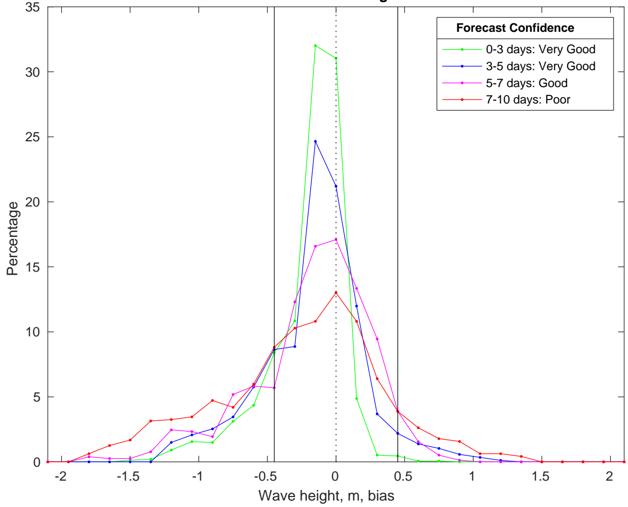
NDBC 42019 vs CMEMS Waves Bias Histogram: 12-Mar-2025
