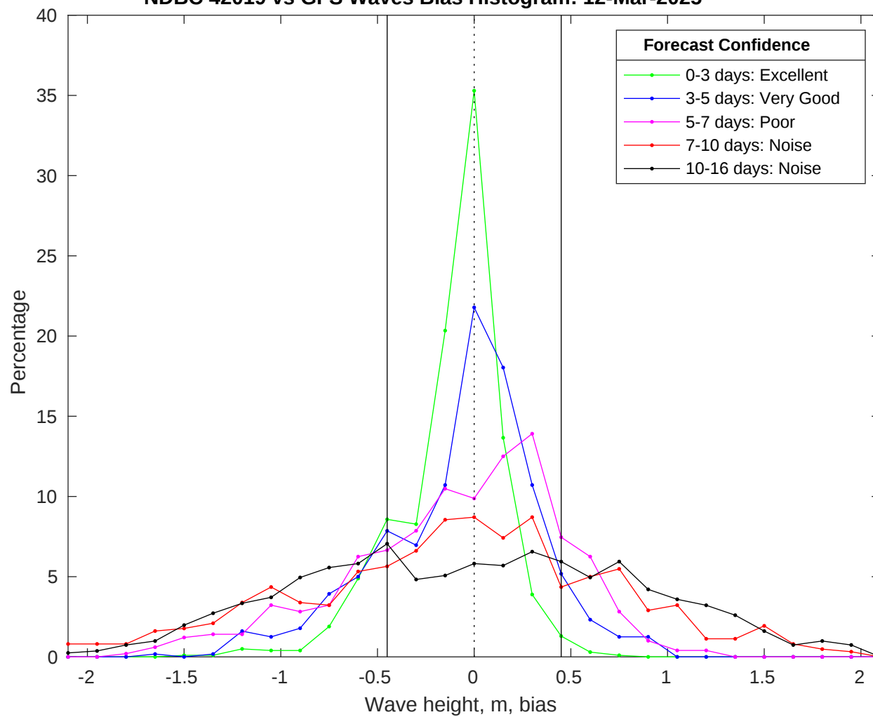
NDBC 42019 vs GFS Waves Bias Histogram: 12-Mar-2025
