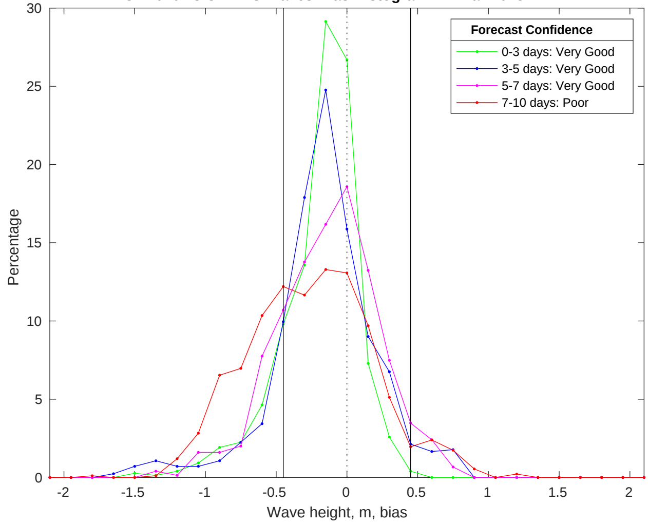
NDBC 42020 vs CMEMS Waves Bias Histogram: 11-Mar-2025
