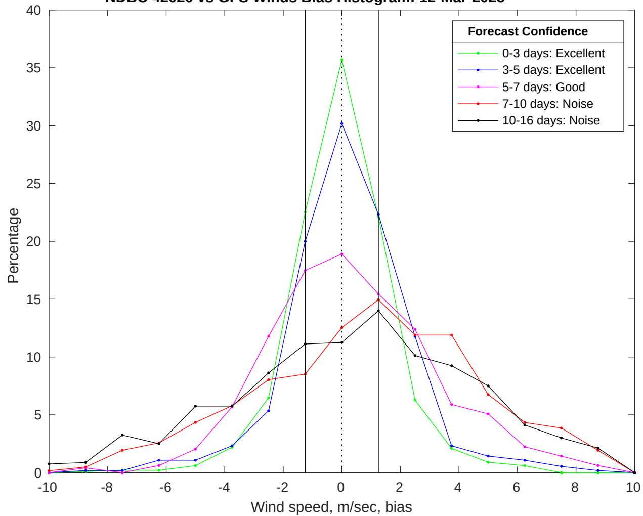
NDBC 42020 vs GFS Winds Bias Histogram: 12-Mar-2025
