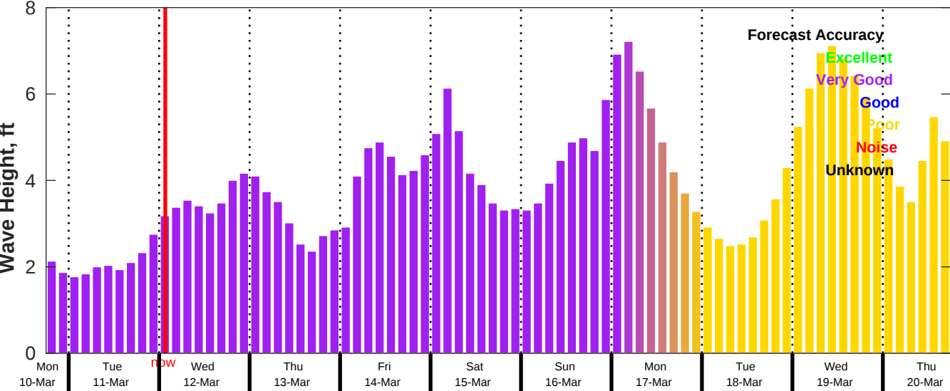
CMEMS Wave Forecast for NDBC 42020 from 10-Mar-2025 18:00:00 to 20-Mar-2025 18:00:00
