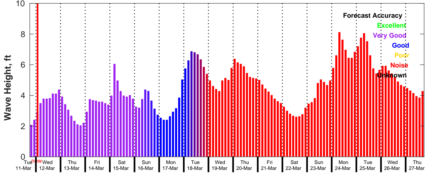
GFS Wave Forecast for NDBC 42020 from 11-Mar-2025 18:00:00 to 27-Mar-2025 18:00:00
