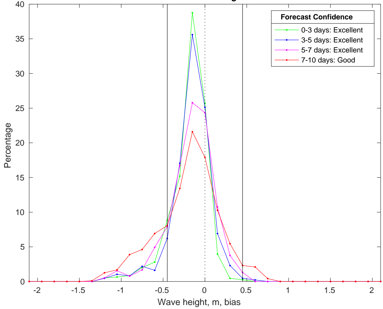
NDBC 42035 vs CMEMS Waves Bias Histogram: 12-Mar-2025
