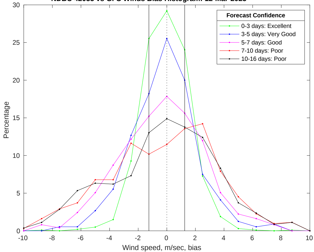
NDBC 42035 vs GFS Winds Bias Histogram: 12-Mar-2025
