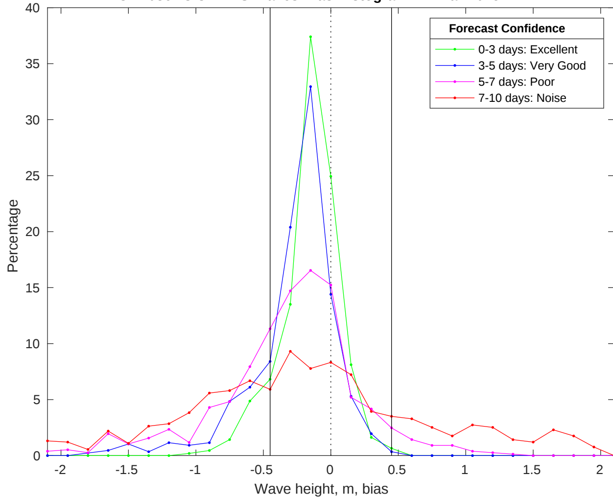
NDBC 42036 vs CMEMS Waves Bias Histogram: 12-Mar-2025
