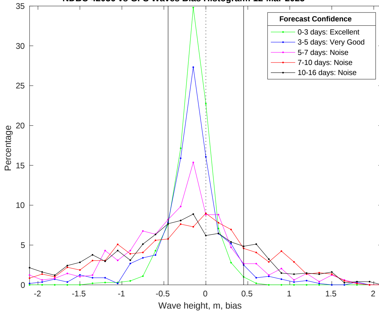
NDBC 42036 vs GFS Waves Bias Histogram: 12-Mar-2025
