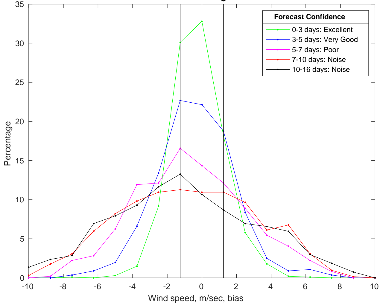
NDBC 42036 vs GFS Winds Bias Histogram: 12-Mar-2025
