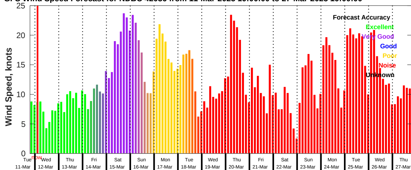
GFS Wind Speed Forecast for NDBC 42036 from 11-Mar-2025 19:00:00 to 27-Mar-2025 19:00:00
