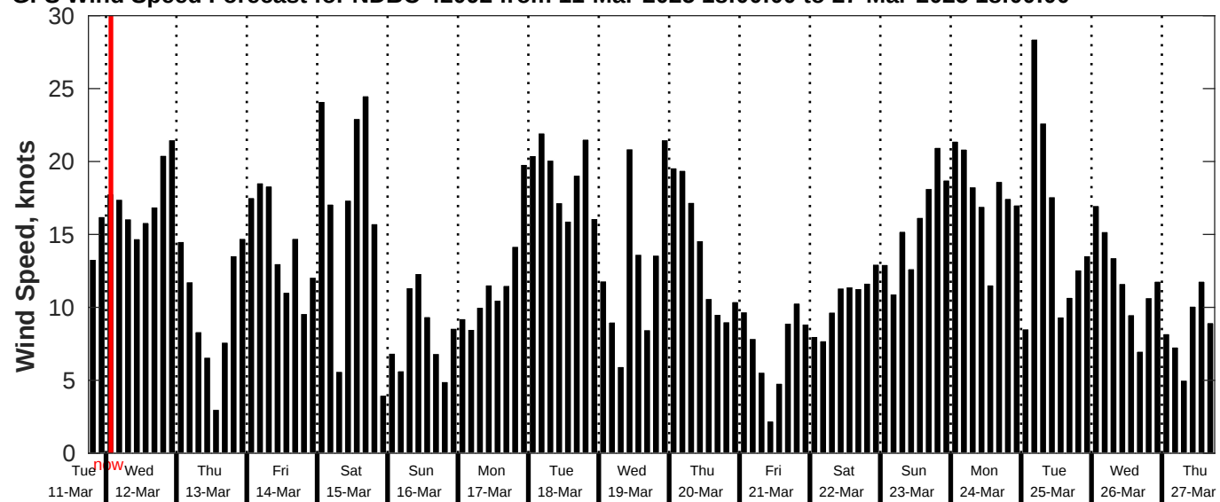
GFS Wind Speed Forecast for NDBC 42092 from 11-Mar-2025 18:00:00 to 27-Mar-2025 18:00:00
