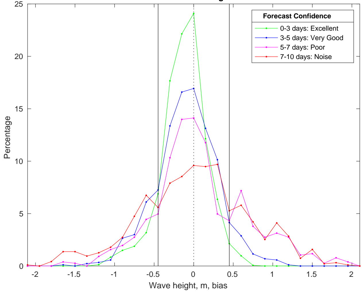
NDBC 46011 vs CMEMS Waves Bias Histogram: 12-Mar-2025
