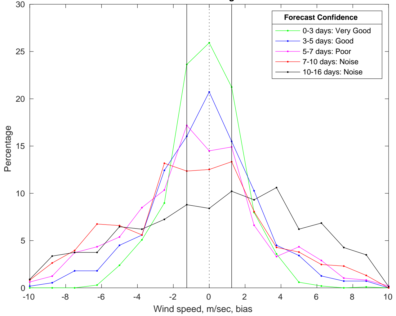
NDBC 46011 vs GFS Winds Bias Histogram: 12-Mar-2025
