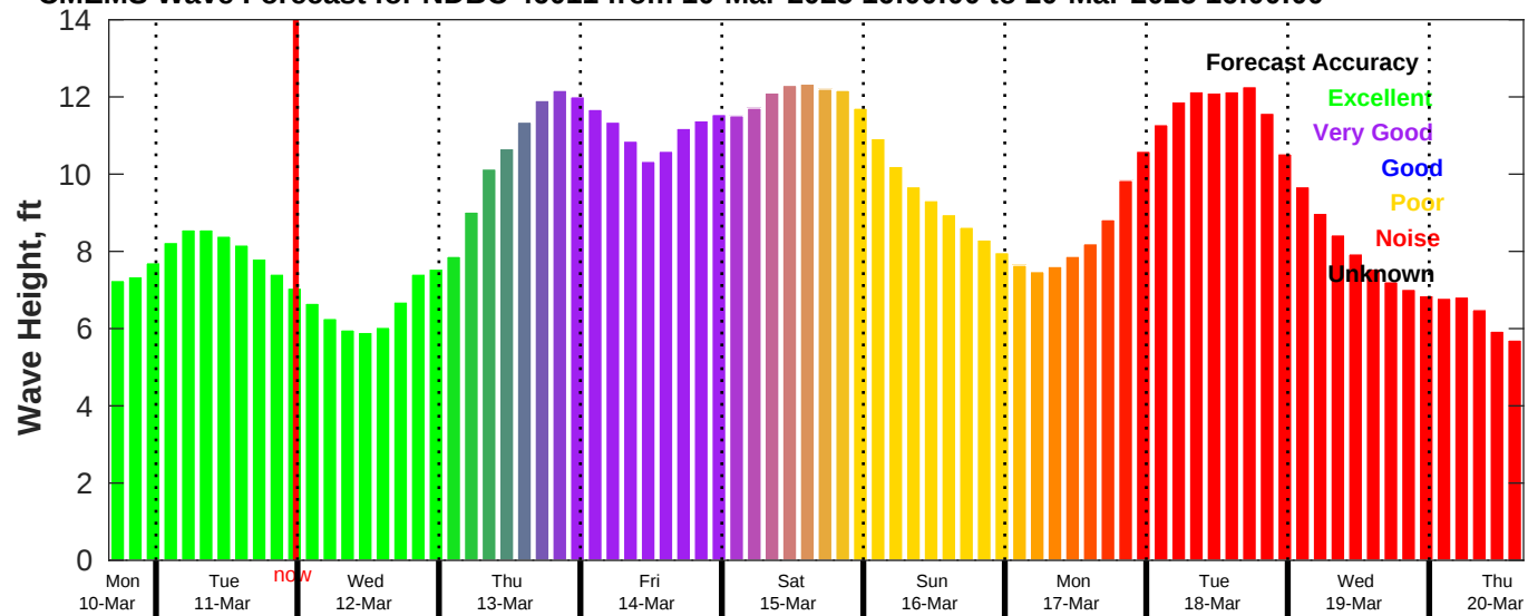
CMEMS Wave Forecast for NDBC 46011 from 10-Mar-2025 16:00:00 to 20-Mar-2025 16:00:00
