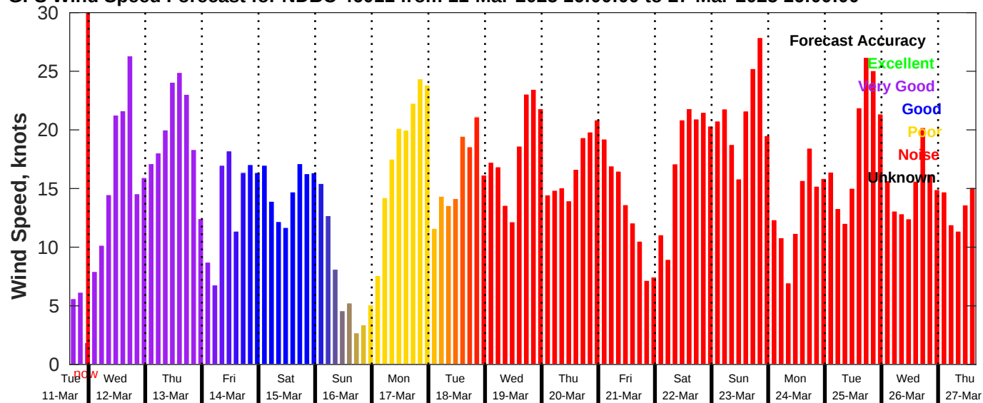
GFS Wind Speed Forecast for NDBC 46011 from 11-Mar-2025 16:00:00 to 27-Mar-2025 16:00:00
