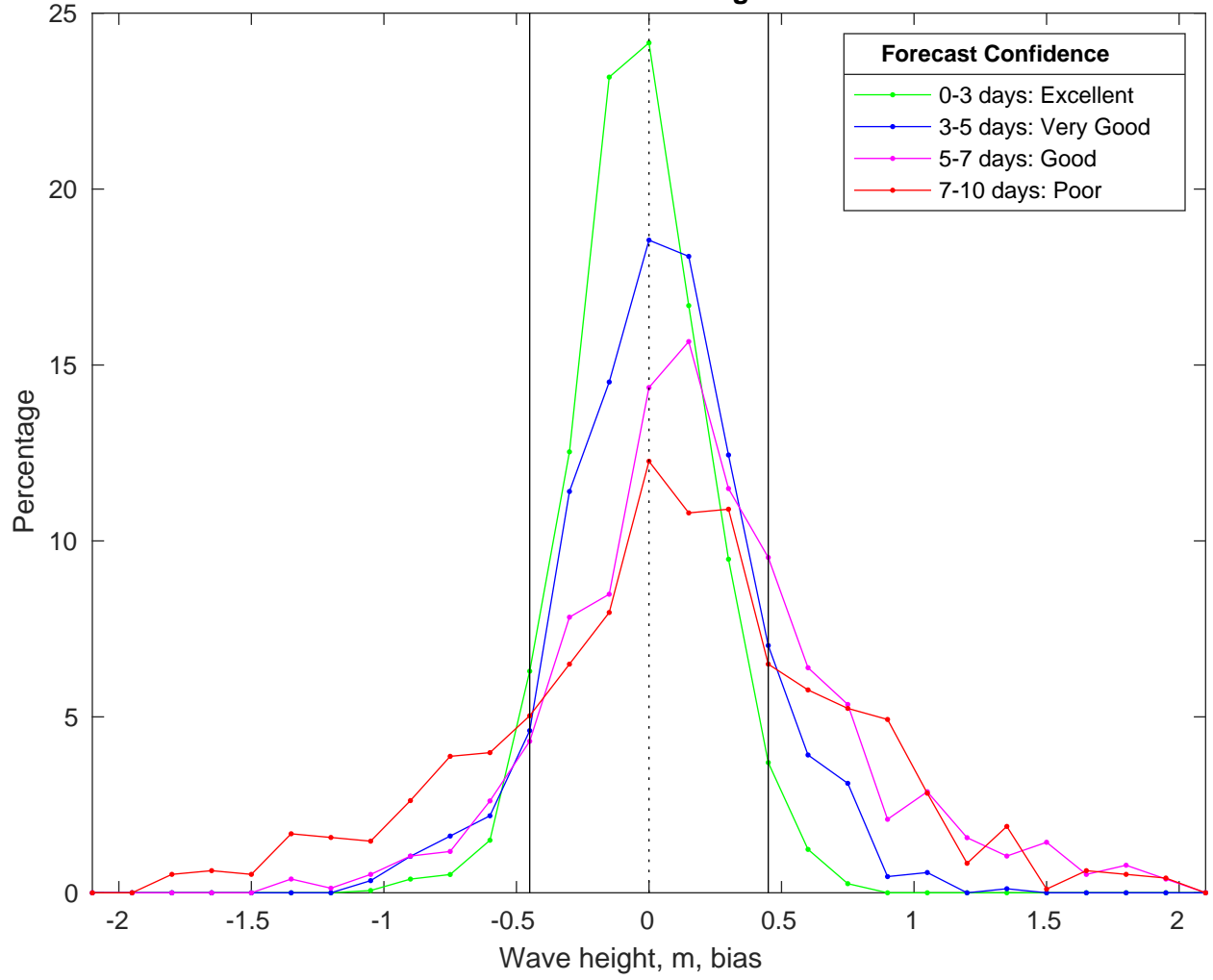
NDBC 46028 vs CMEMS Waves Bias Histogram: 12-Mar-2025
