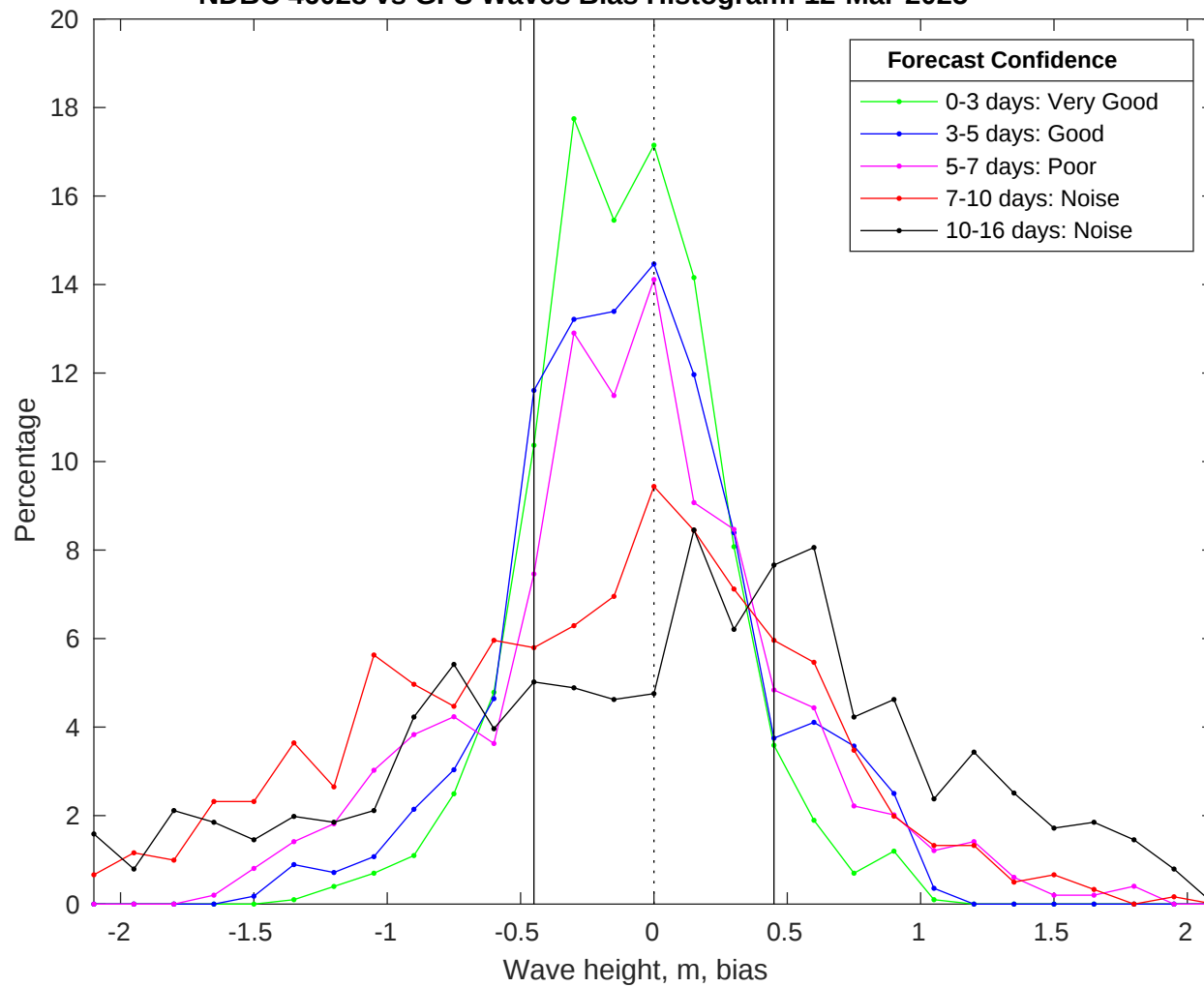
NDBC 46028 vs GFS Waves Bias Histogram: 12-Mar-2025
