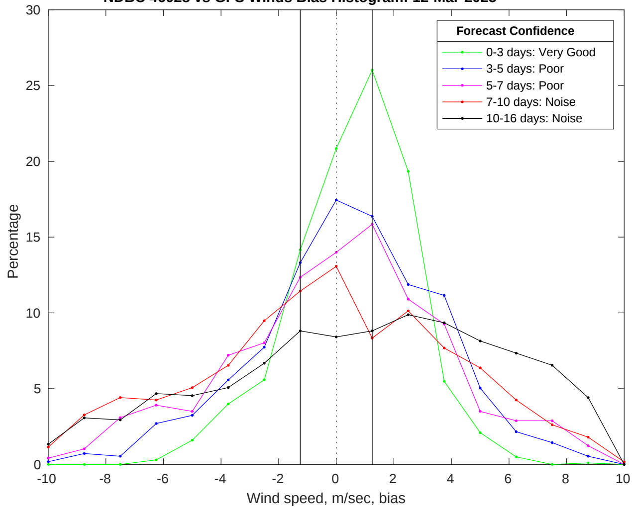
NDBC 46028 vs GFS Winds Bias Histogram: 12-Mar-2025
