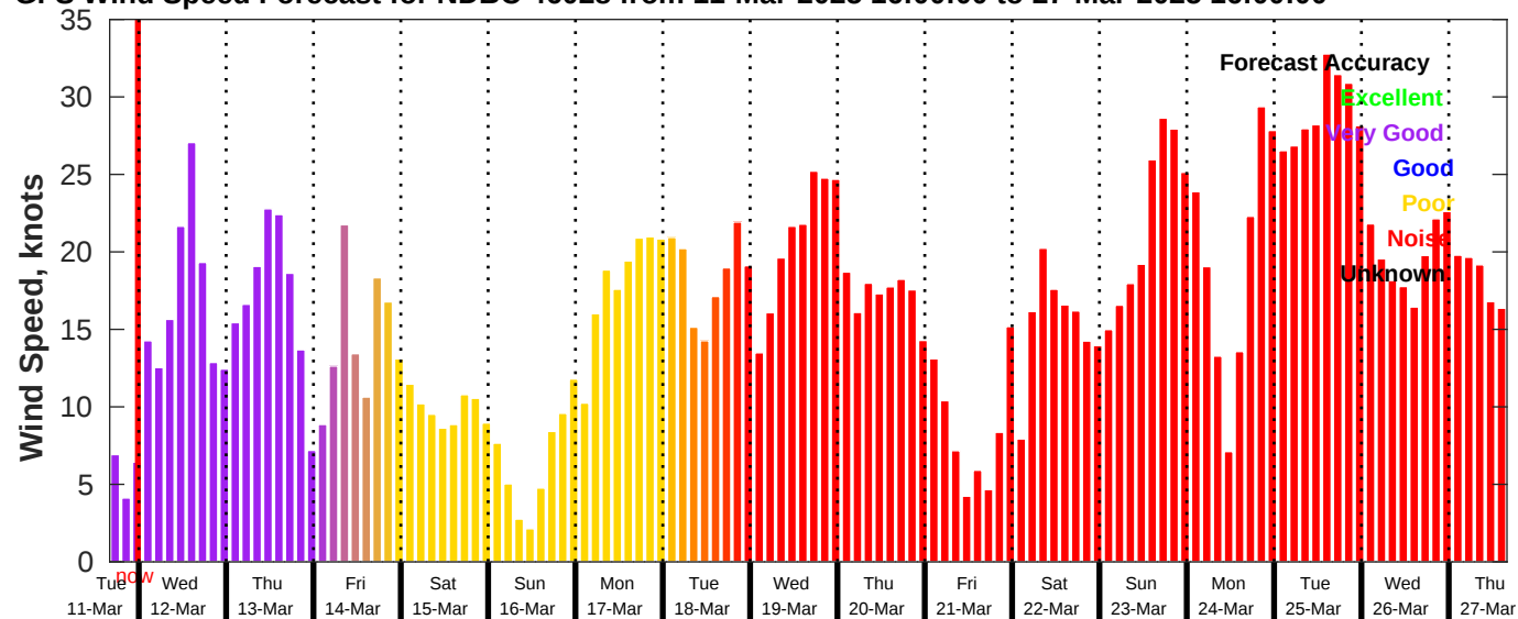
GFS Wind Speed Forecast for NDBC 46028 from 11-Mar-2025 16:00:00 to 27-Mar-2025 16:00:00
