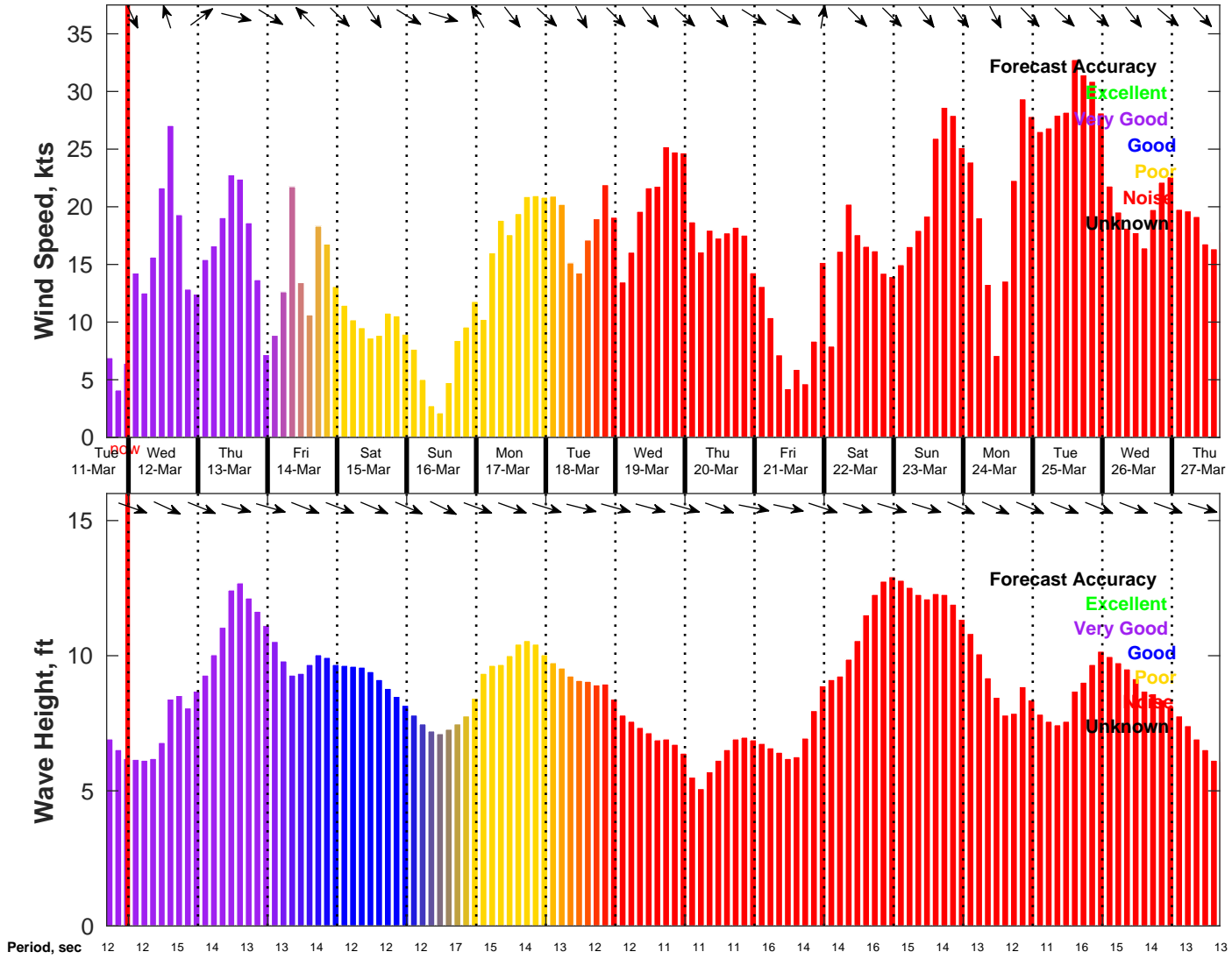
Wind & Wave Forecast for NDBC 46028 from 11-Mar-2025 16:00:00 to 27-Mar-2025 16:00:00
