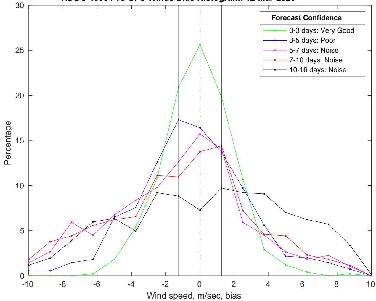
NDBC 46054 vs GFS Winds Bias Histogram: 12-Mar-2025
