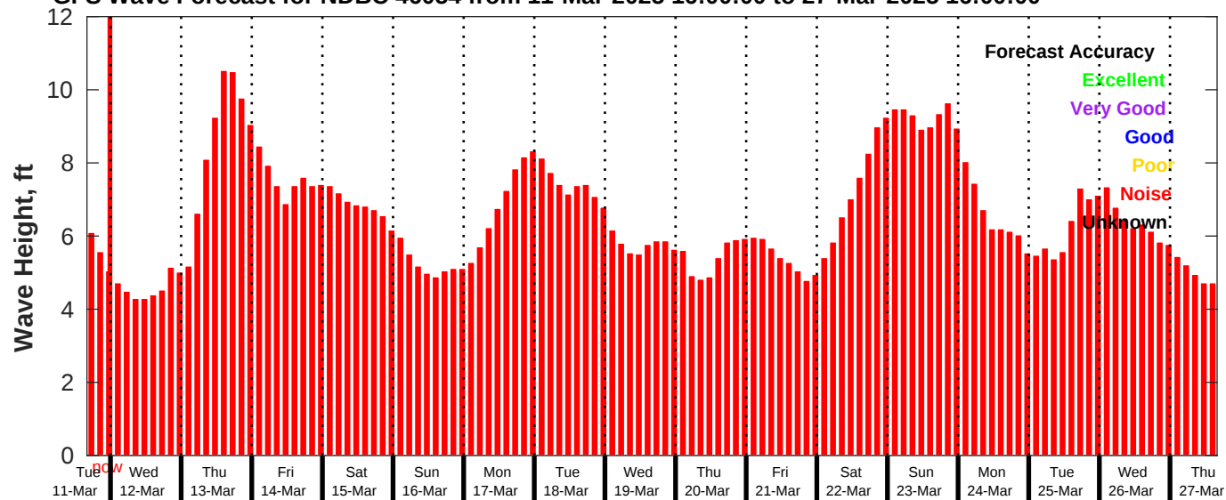
GFS Wave Forecast for NDBC 46054 from 11-Mar-2025 16:00:00 to 27-Mar-2025 16:00:00
