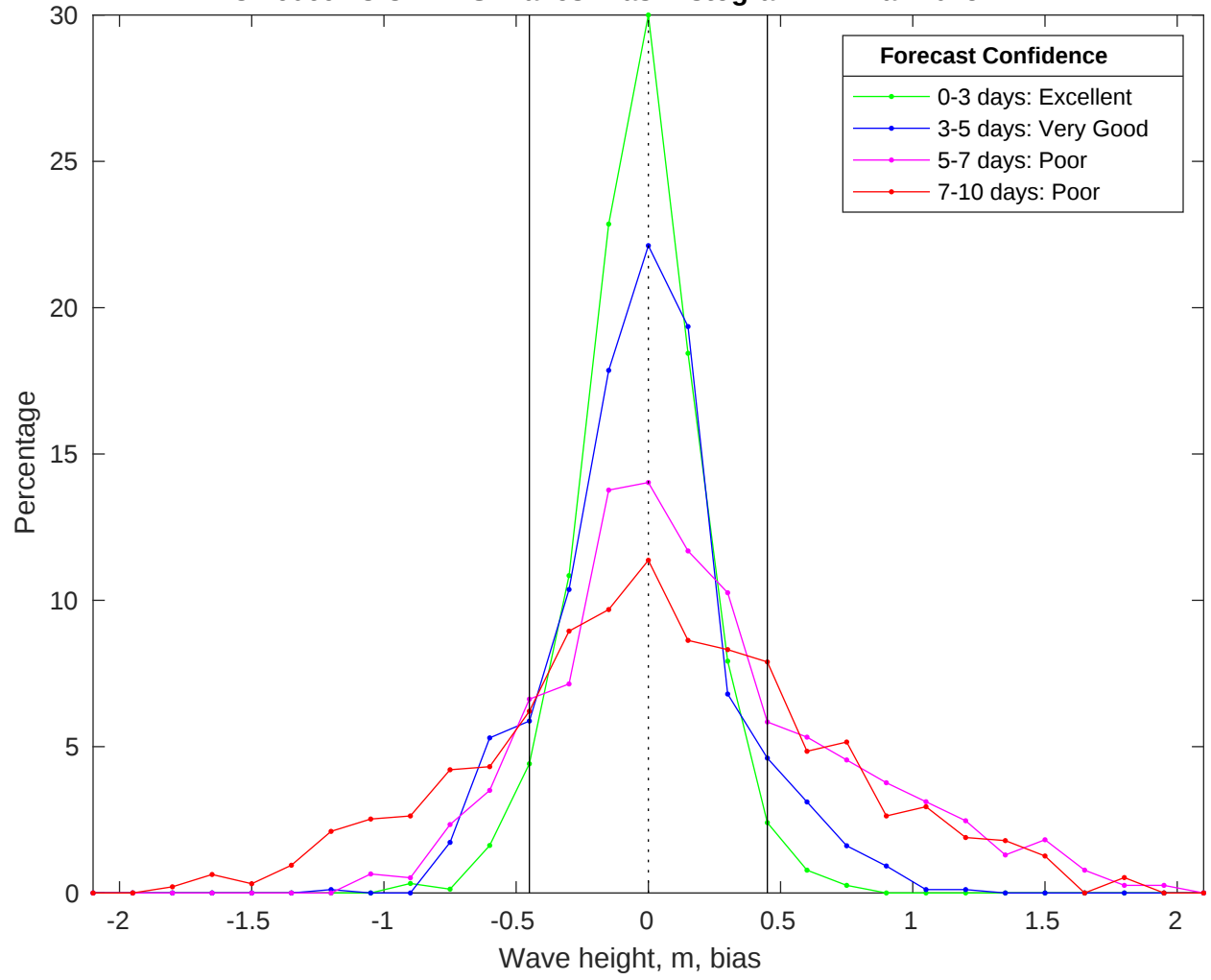
NDBC 46069 vs CMEMS Waves Bias Histogram: 12-Mar-2025
