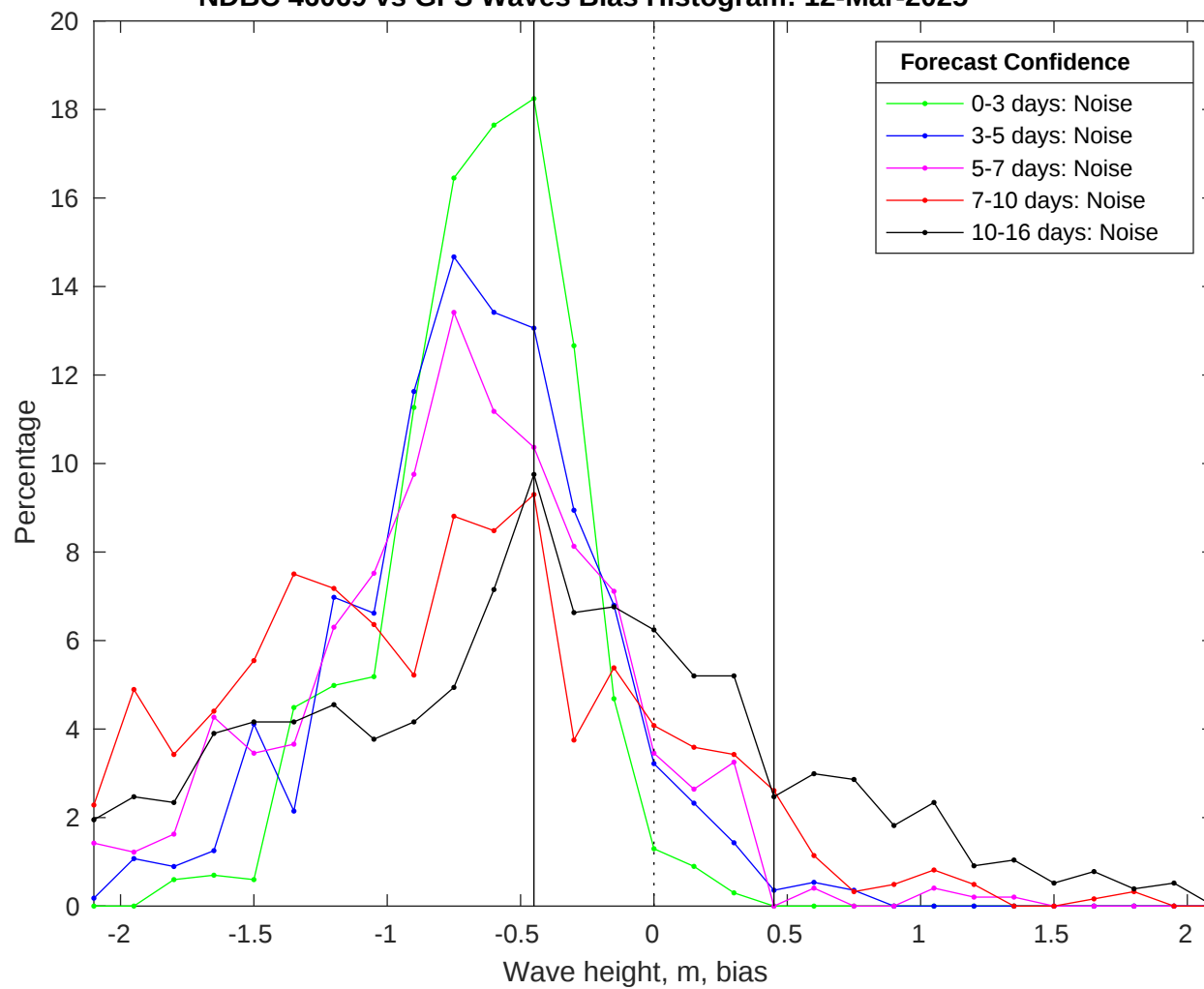
NDBC 46069 vs GFS Waves Bias Histogram: 12-Mar-2025
