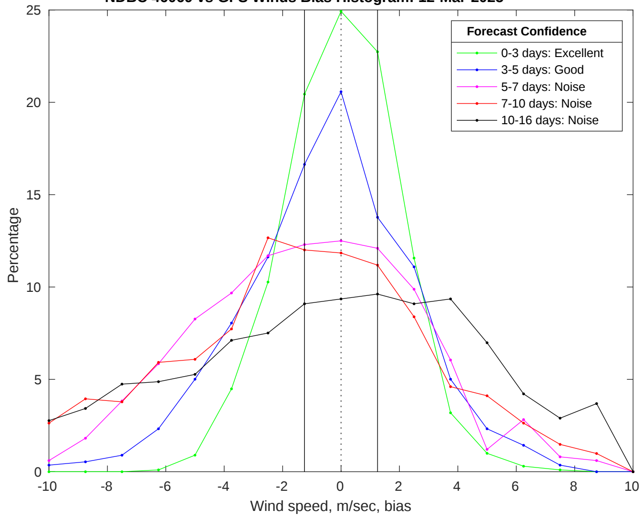
NDBC 46069 vs GFS Winds Bias Histogram: 12-Mar-2025
