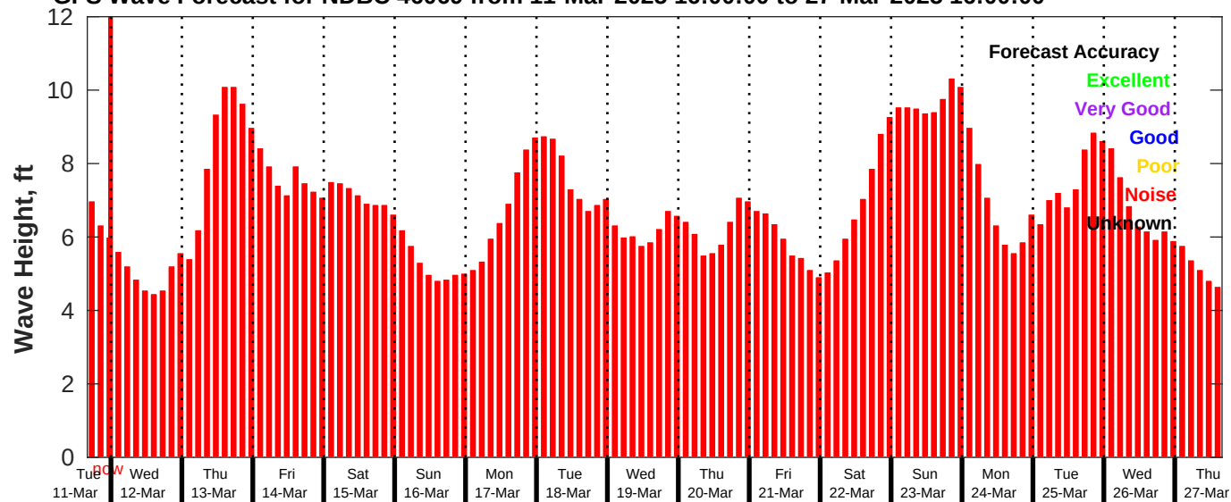
GFS Wave Forecast for NDBC 46069 from 11-Mar-2025 16:00:00 to 27-Mar-2025 16:00:00
