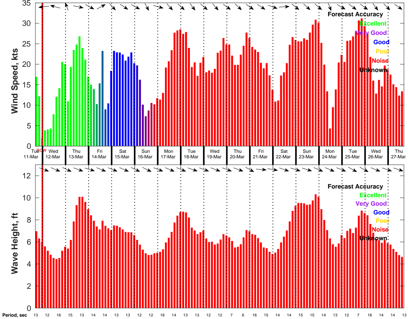
Wind & Wave Forecast for NDBC 46069 from 11-Mar-2025 16:00:00 to 27-Mar-2025 16:00:00
