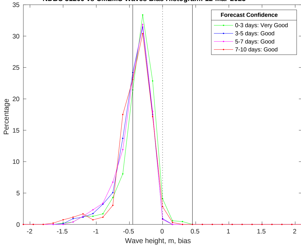
NDBC 51209 vs CMEMS Waves Bias Histogram: 12-Mar-2025
