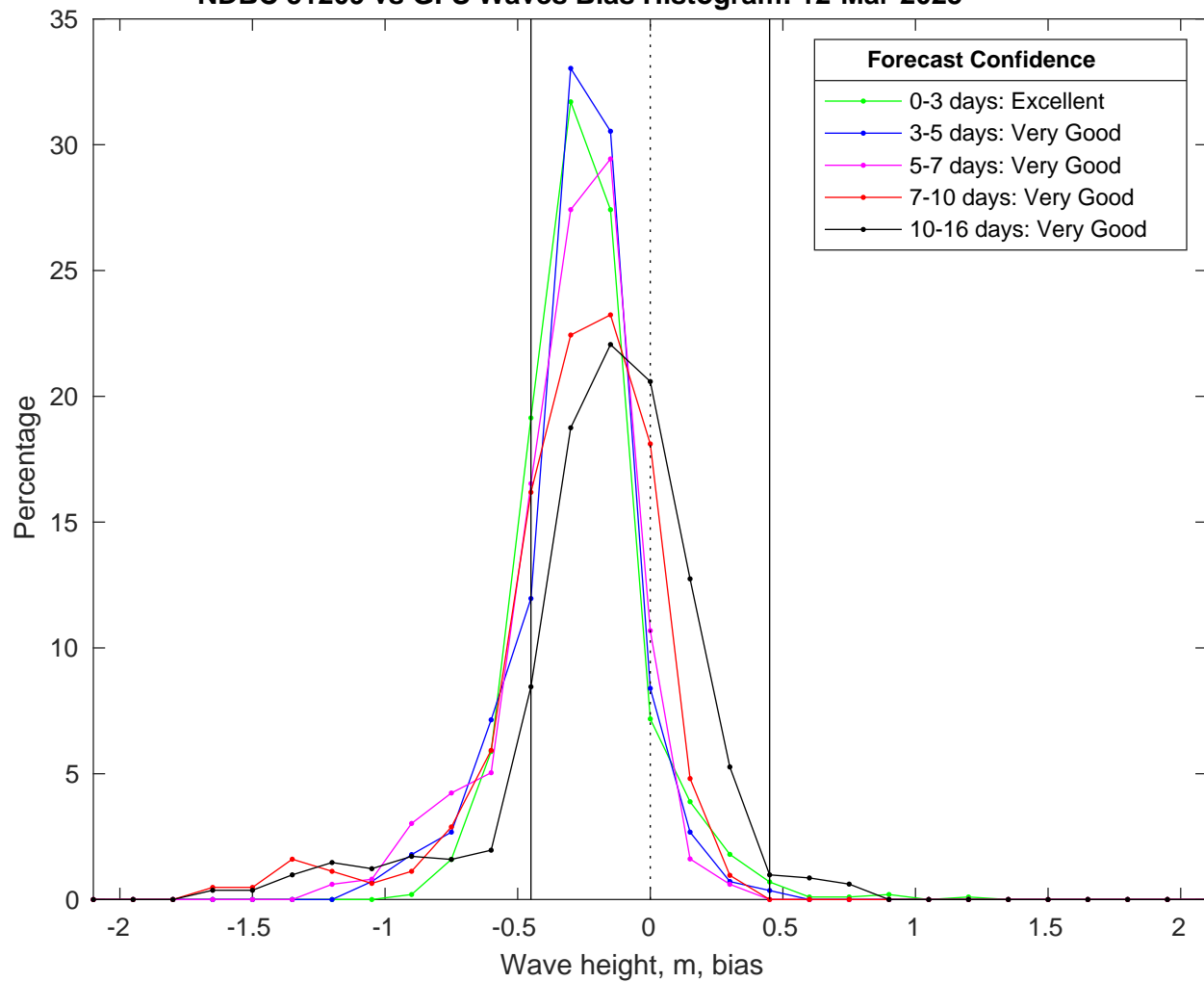
NDBC 51209 vs GFS Waves Bias Histogram: 12-Mar-2025
