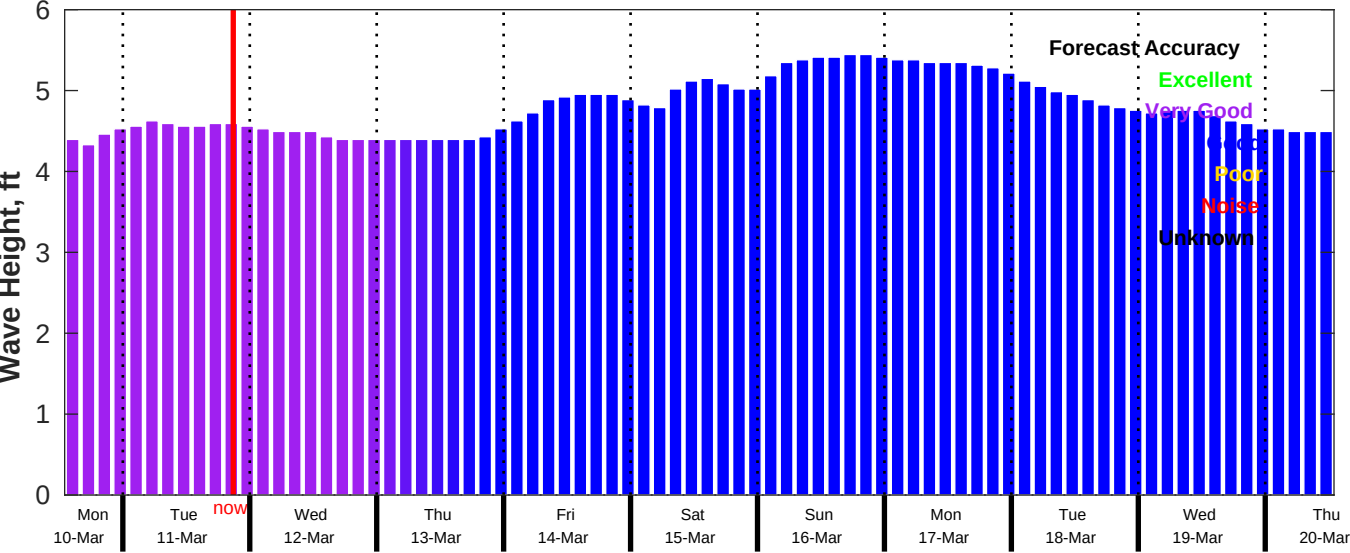
CMEMS Wave Forecast for NDBC 51209 from 10-Mar-2025 13:00:00 to 20-Mar-2025 13:00:00
