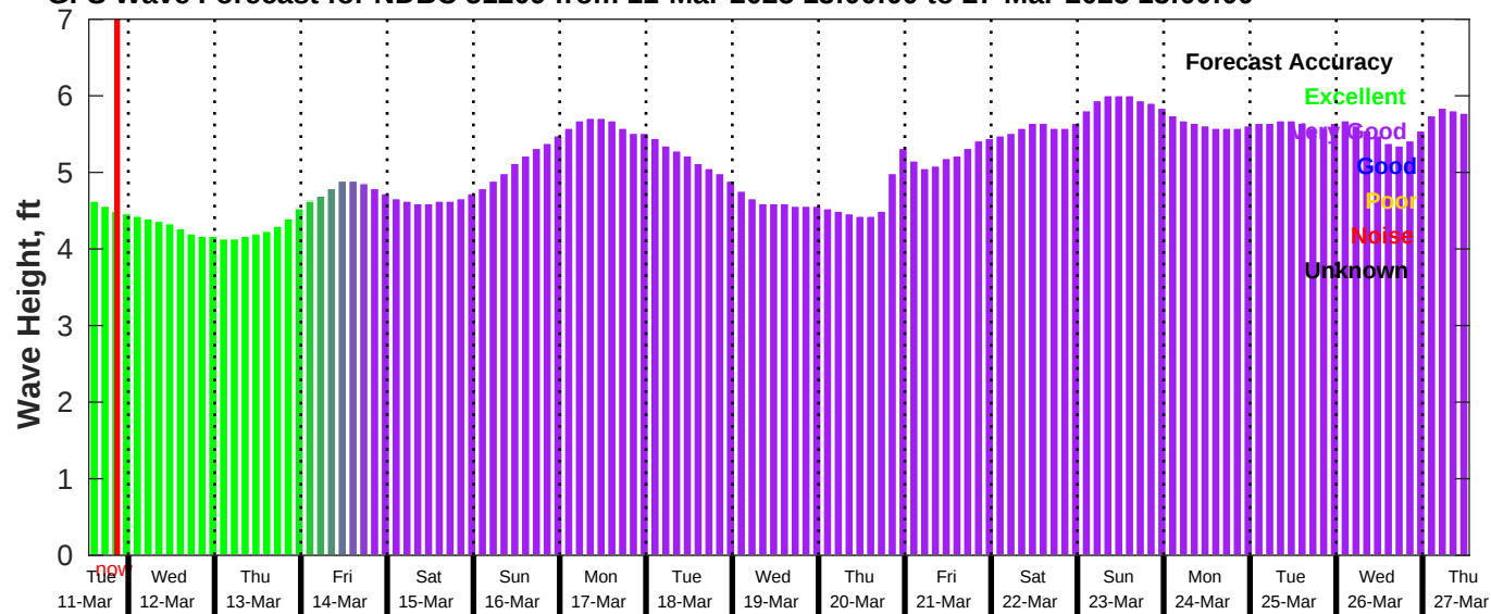
GFS Wave Forecast for NDBC 51209 from 11-Mar-2025 13:00:00 to 27-Mar-2025 13:00:00
