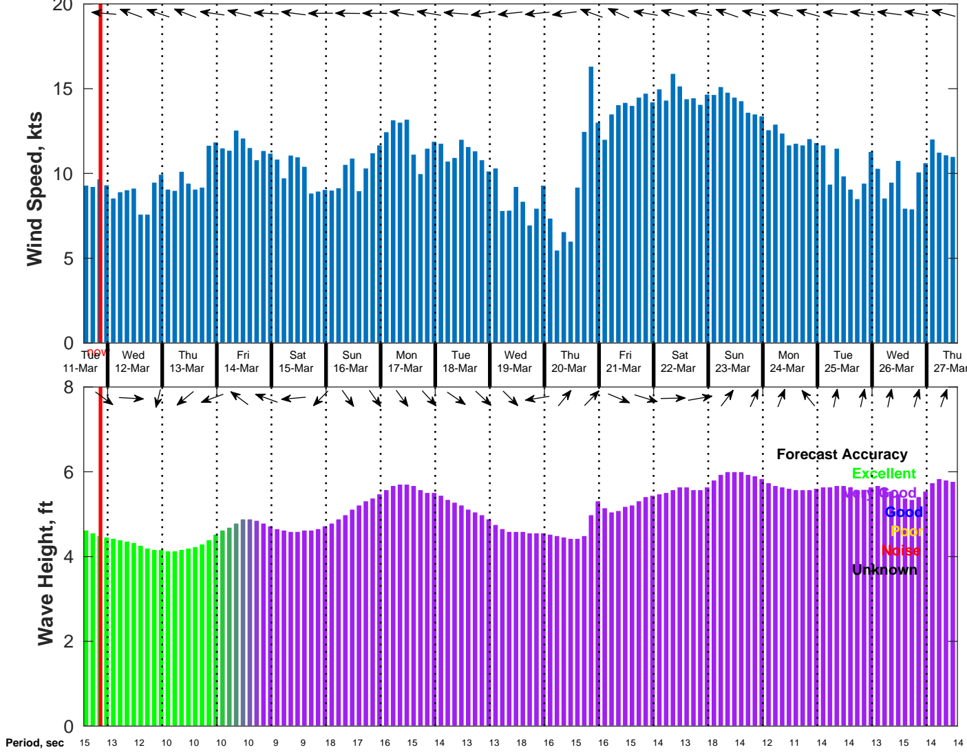
Wind & Wave Forecast for NDBC 51209 from 11-Mar-2025 13:00:00 to 27-Mar-2025 13:00:00
