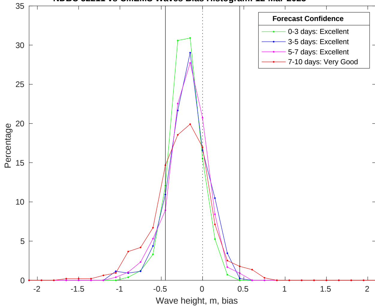
NDBC 52211 vs CMEMS Waves Bias Histogram: 12-Mar-2025
