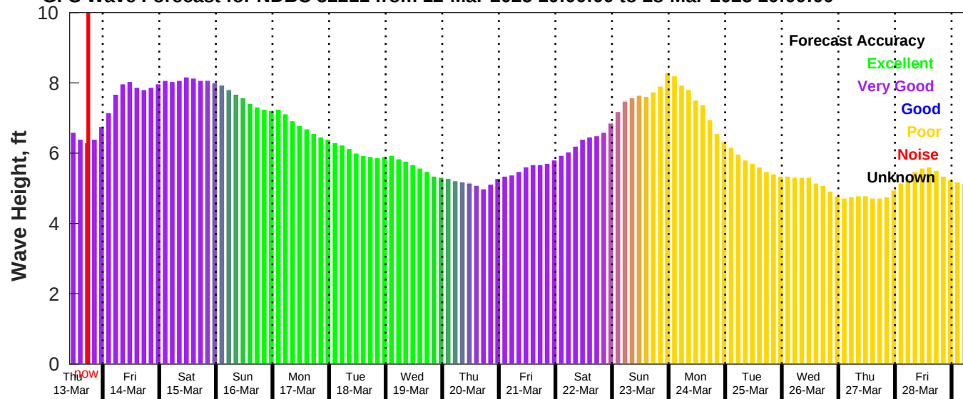
GFS Wave Forecast for NDBC 52211 from 12-Mar-2025 10:00:00 to 28-Mar-2025 10:00:00
