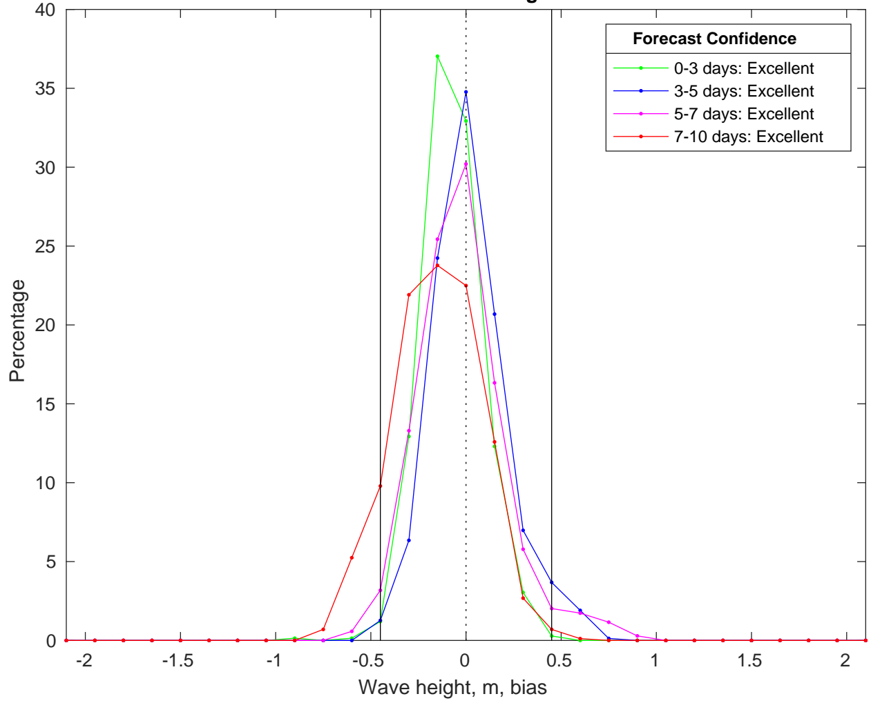
NDBC 52212 vs CMEMS Waves Bias Histogram: 12-Mar-2025
