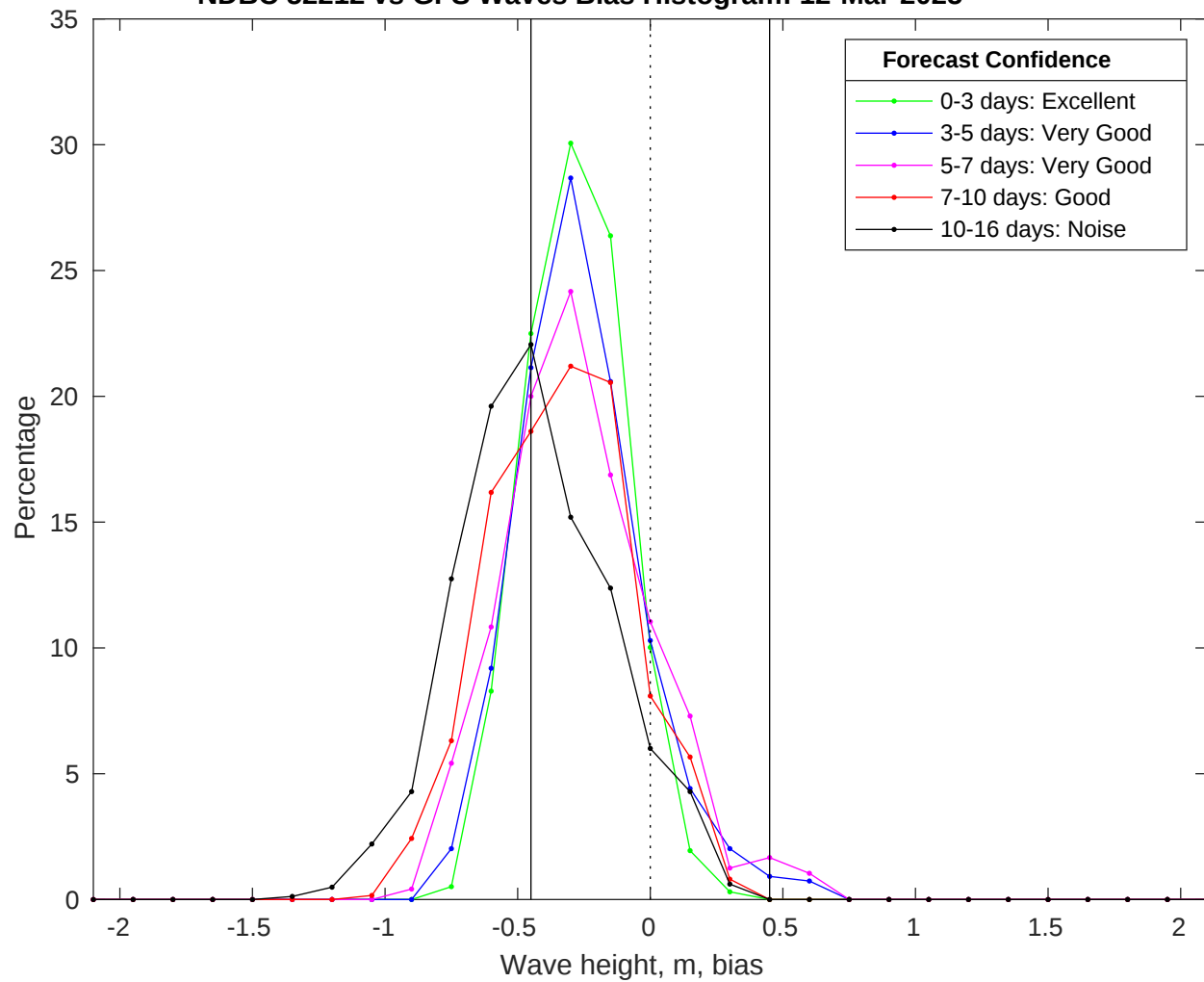
NDBC 52212 vs GFS Waves Bias Histogram: 12-Mar-2025
