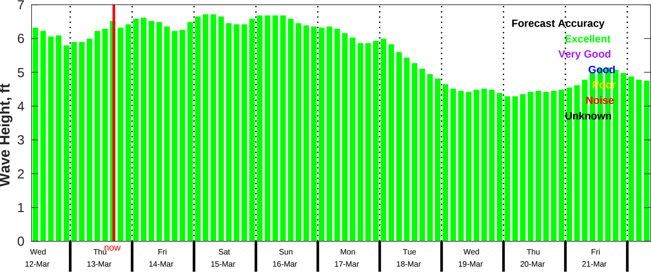
CMEMS Wave Forecast for NDBC 52212 from 11-Mar-2025 09:00:00 to 21-Mar-2025 09:00:00
