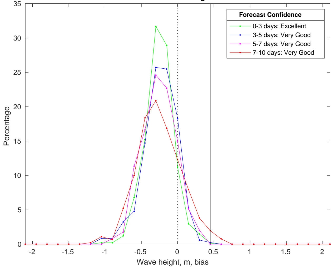
NDBC 52213 vs CMEMS Waves Bias Histogram: 12-Mar-2025
