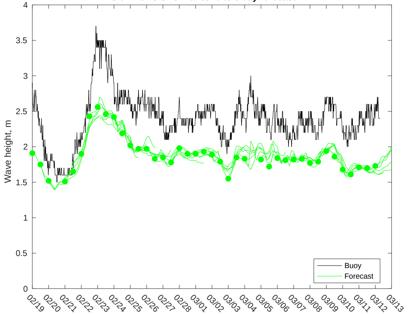
NDBC 52213 vs GFS Waves: 0 to 3 day forecast
