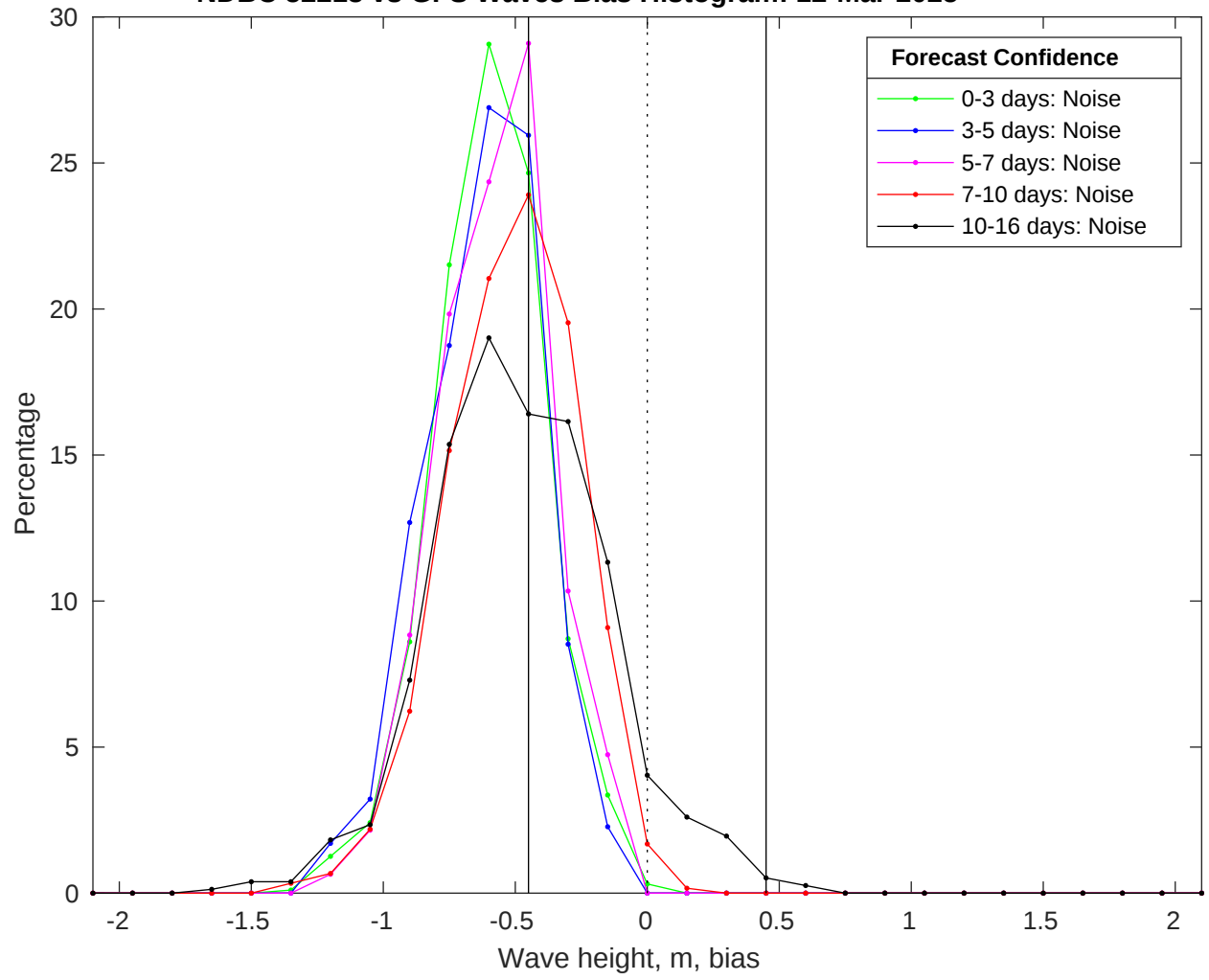
NDBC 52213 vs GFS Waves Bias Histogram: 12-Mar-2025
