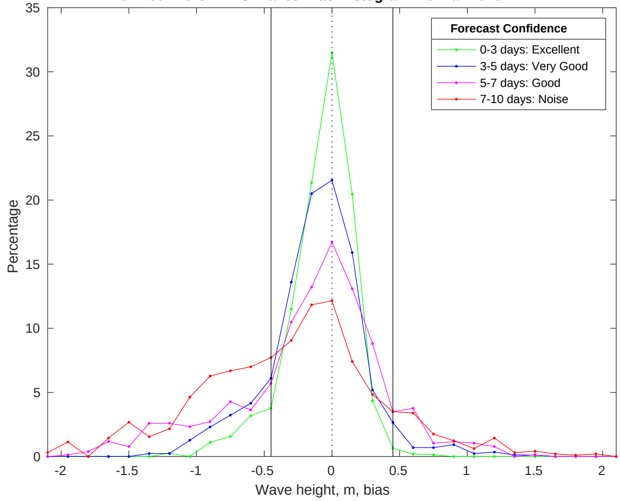
NDBC 41004 vs CMEMS Waves Bias Histogram: 13-Mar-2025
