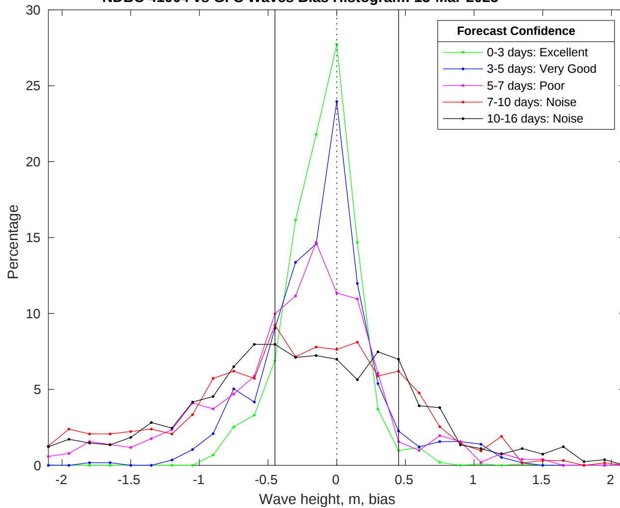
NDBC 41004 vs GFS Waves Bias Histogram: 13-Mar-2025
