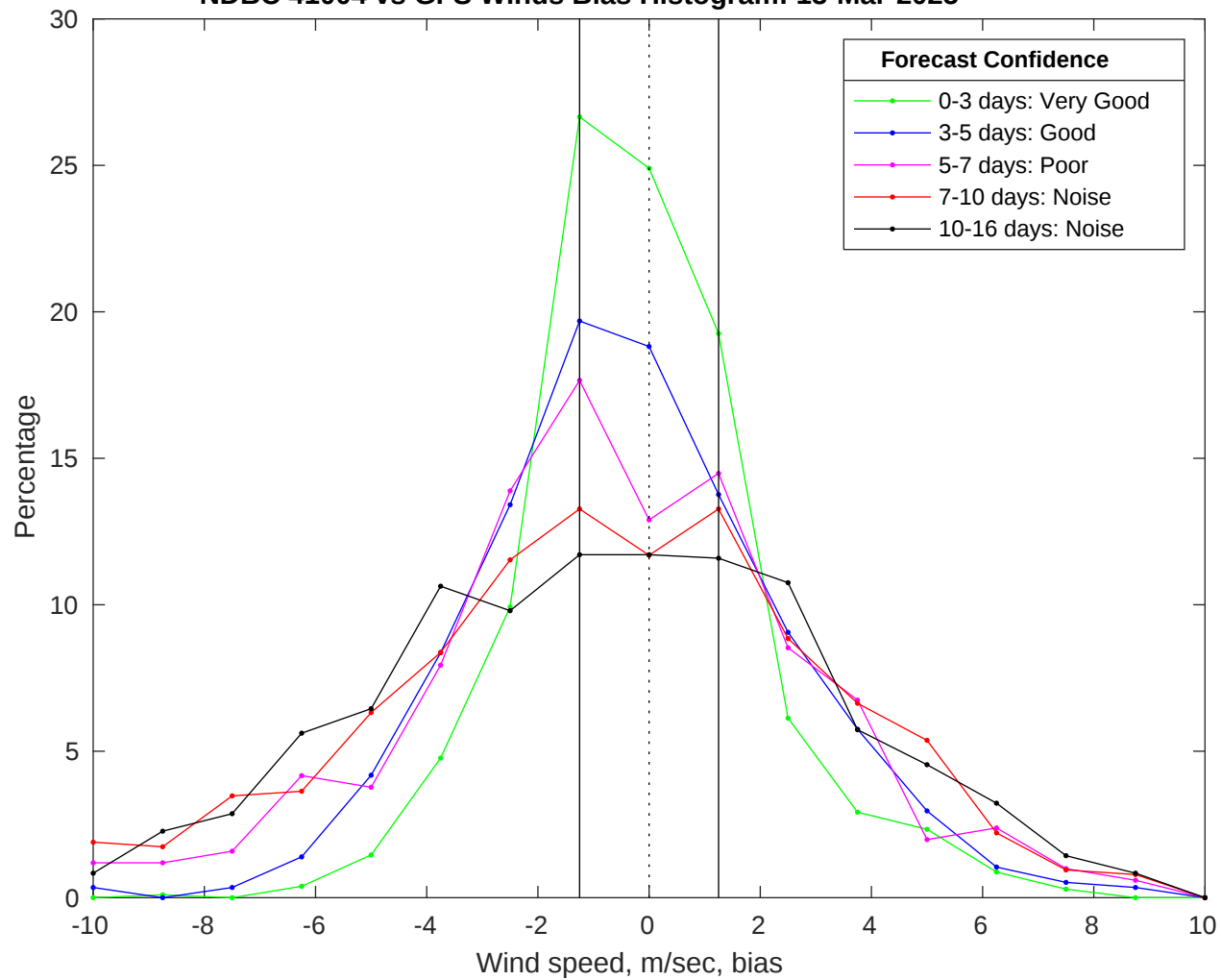
NDBC 41004 vs GFS Winds Bias Histogram: 13-Mar-2025
